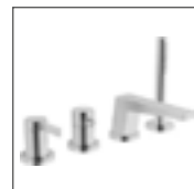
HANSA LOFT trim kit single-lever mixer for all 4-hole installation units* 5775 2073 chrome suitable for installation unit 53020200 / 53040200 / 53080200 projection: 185 mm
