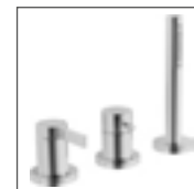
HANSA LOFT trim kit single-lever mixer for all 3-hole installation units* 5779 9073 chrome for distant positioned bathtub spout (HANSAFILL), without HANSAFILL tub filler and drain assembly
