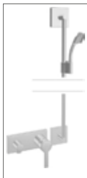
HANSARONDA trim kit single-lever mixer, DN 15 suitable for HANSAMATRIX installation unit* 4487 2010 chrome with solid-metal shower bar 1100 mm
