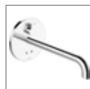
HANSAELECTRA trim kit with function unit concealed electronic mixer, DN 15 (G1/2) with temperature mixing device suitable for HANSABLUEBOX concealed unit* 8081 2121 chrome projection: 310 mm
