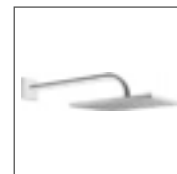
HANSAVIVA overhead shower, DN 15 for wall-mounting 0418 0340 chrome shower head square 250 x 250 mm projection: 400 mm
